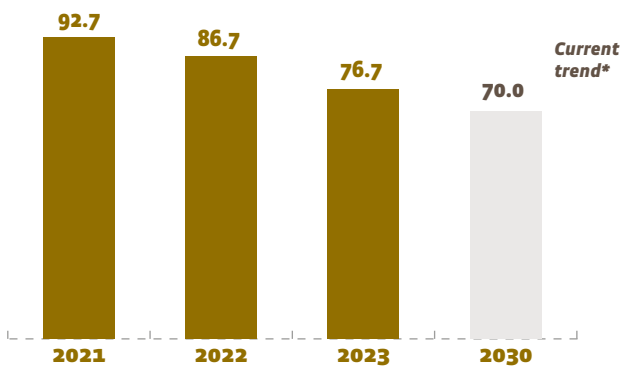
Graph. n° 3 EurObserv'ER projection of electricity production from solid biofuels* in the EU 27 (in TWh)
